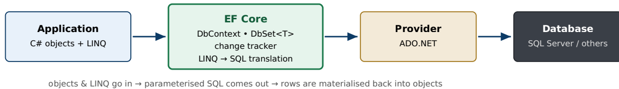
Fig 3.2: EF Core sits between application objects and the relational database
