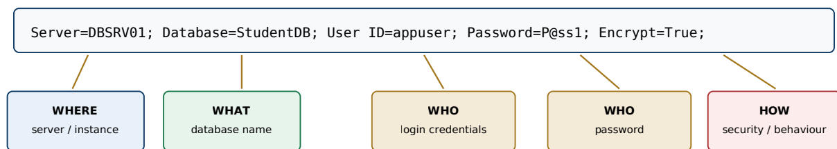
Fig 2.2: Anatomy of a SQL Server connection string
